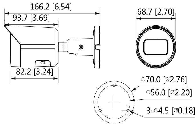
Dimensions (mm[inch])
